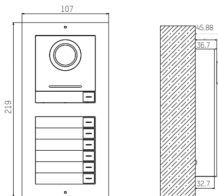
Dual Modules Surface Mounting
